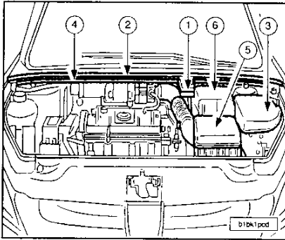
Motor TU3JP.
