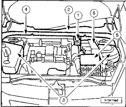
Motor TU5JP4.
