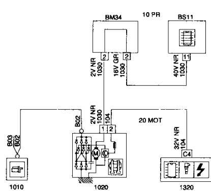
1020 ALTERNADOR (MOTOR TU3JP)
