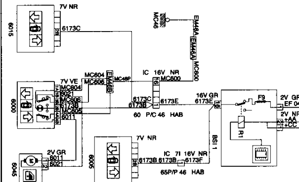
6000 CONTACTOR ELEVALUNAS CONDUCTOR PUERTA CONDUCTOR
