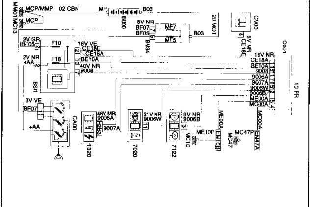
C001 CONECTOR DIAGNOSIS
